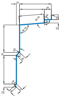
STD. HOOD TRIM
