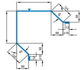
STD. OUTSIDE CORNER TRIM
