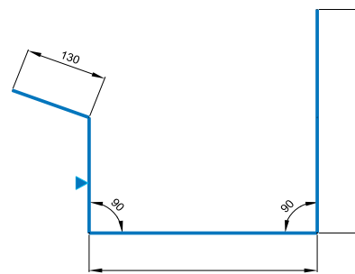
EAVE GUTTER
