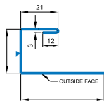
STD. PANEL END CLOSURE TRIM
