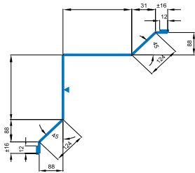
STD. OUTSIDE CORNER TRIM
