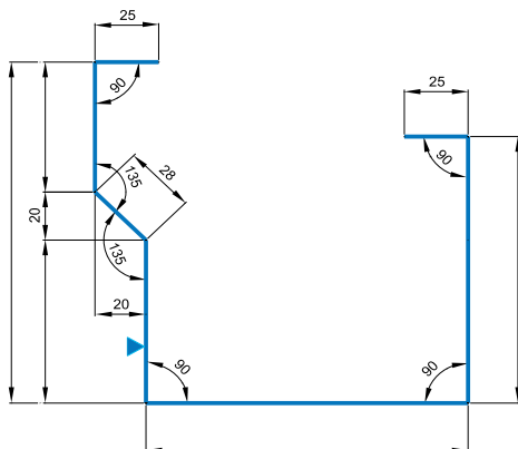
STD. EAVE GUTTER
