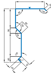
STD. GABLE TRIM
